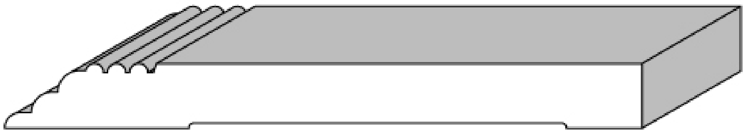
CMK 320 (9/16 x 5-1/2")
