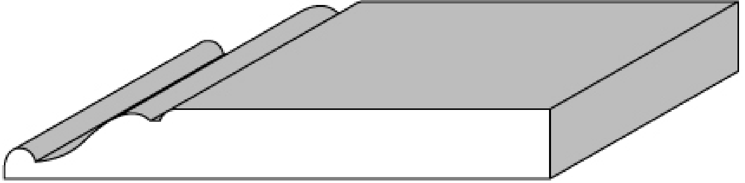
CMK 326 (3/4" x 5-3/8")
