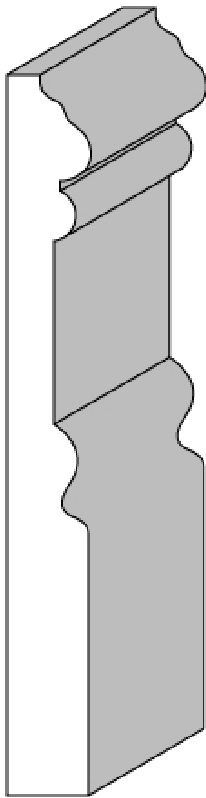
CMK 314 (5/8" x 5-1/2")
