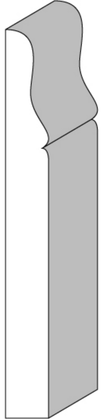
CMK 323 (3/4" x 6-3/4")
